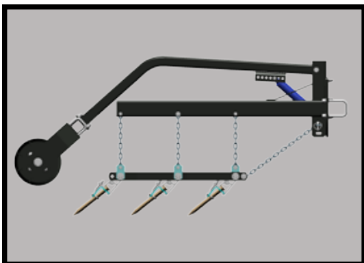
3 Bar Chain with Single Rolling Basket (Also available 3 Bar Coil with Single Rolling Basket)
