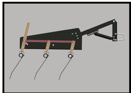
3 Bar Coil Tine Harrow with 3/8" x 18" (9.53mm x 457.2mm) Coil Tines with Simple Angle Adjustability
