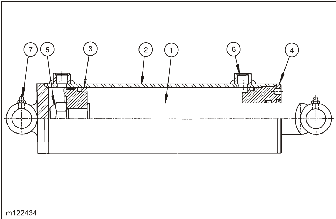
Figure 1-16 4 x 10 Hydraulic Cylinder Assembly
