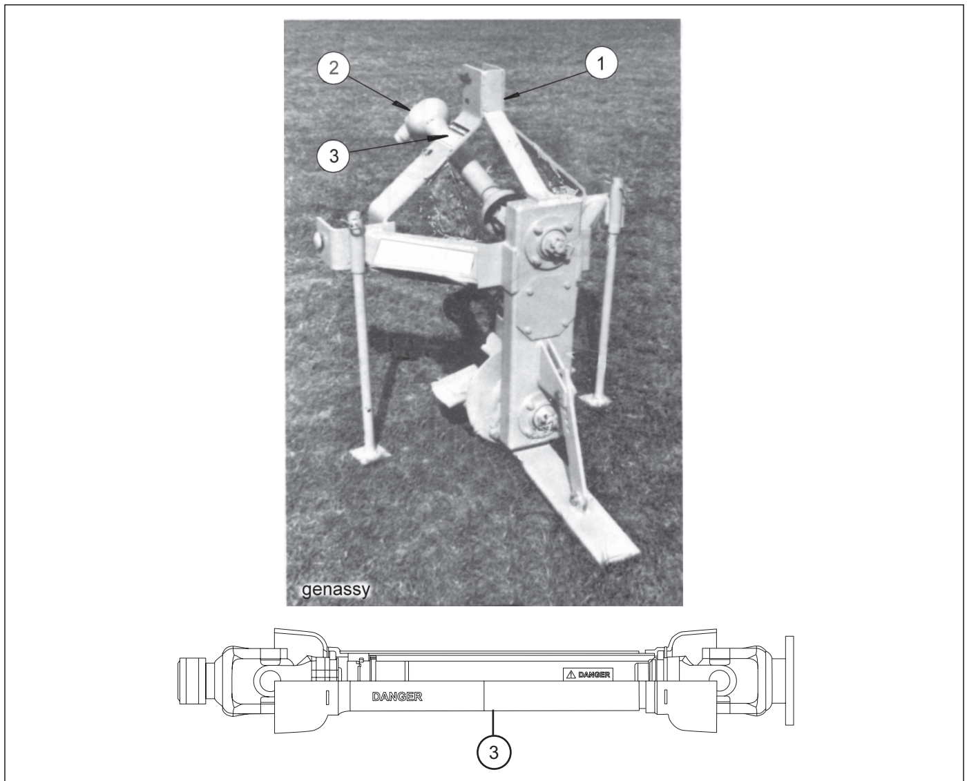
Figure 1-1: General Assembly
