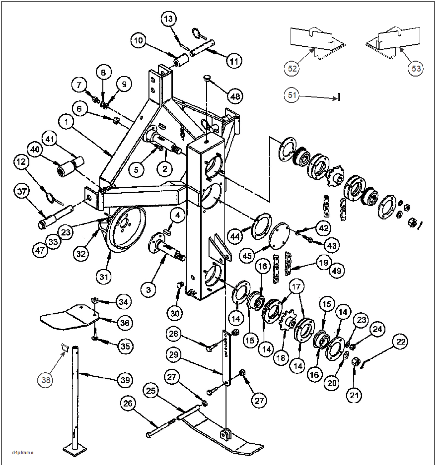
Figure 1-2: Main Frame Assembly
