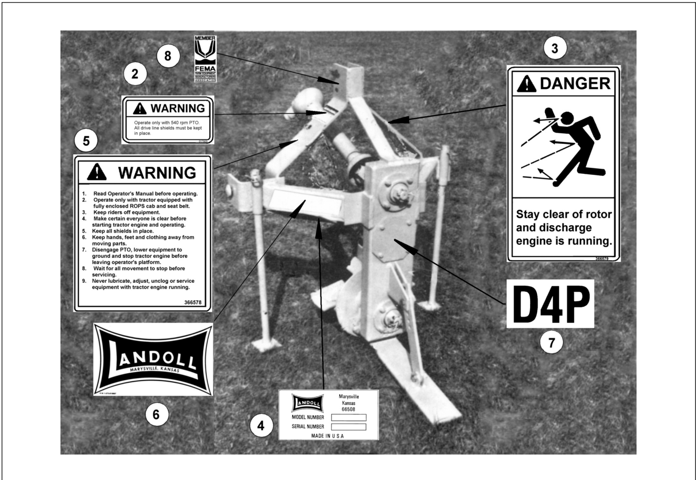
Figure 1-3: Decal Installation
